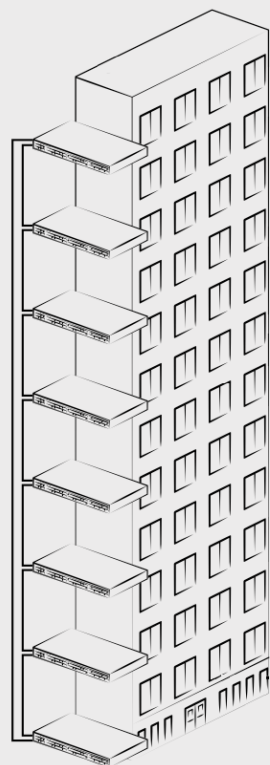
Figure 2. Long distance stacking A stack of ICX switches deployed in a tall building making use of standard SFP+ or QSFP+ optical transceivers and fiber as stacking links. A single stack can cover the entire building simplifying network deployment and management significantly
